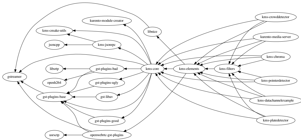
Fig. 1: Media Server dependency graph
