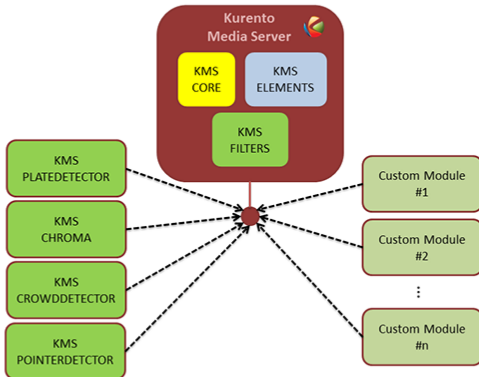
Fig. 6: Kurento modules architecture Kurento Media Server can be extended with built-in modules ( crowddetector , pointerdetector , chroma , platedetector ) and also with other custom modules.
